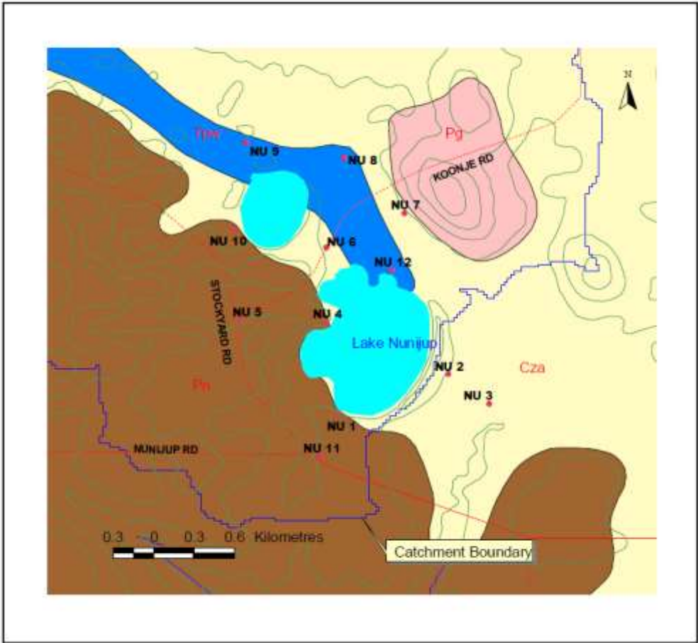
Figure 6: Hydrogeology of Lake Nunijup 9 : Cza – Superficial aquifer Cainozoic sediments, Tpw – Paleochannel sediments, Werillup Formation, Pg – Proterozoic granites, Pn – Fractured and weathered Proterozoic gneisses.
